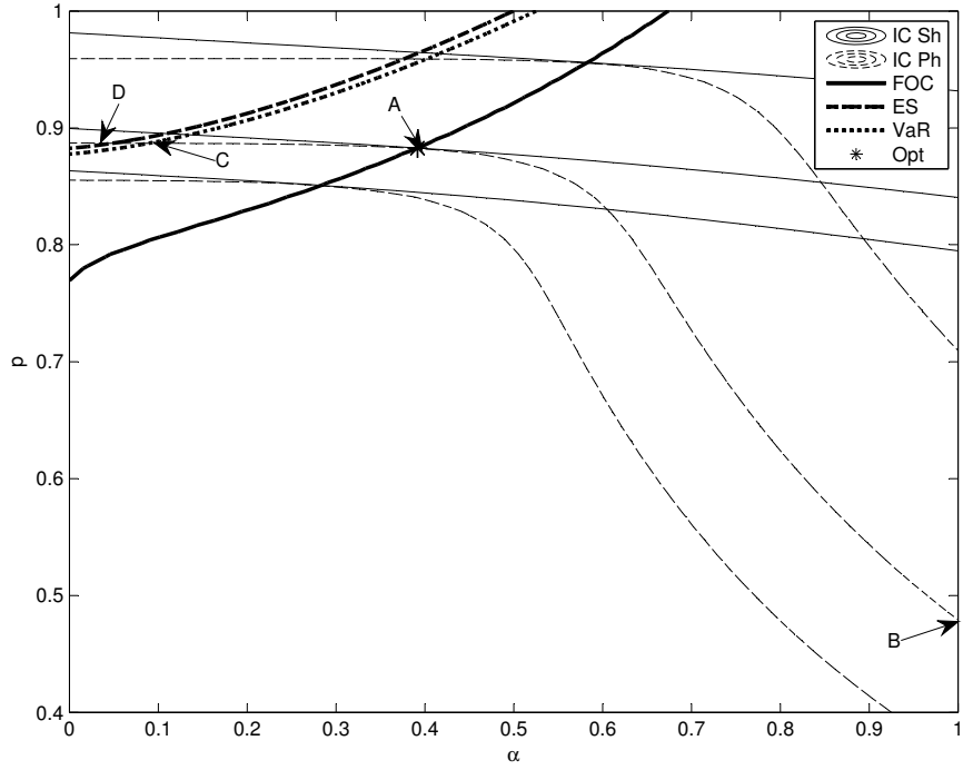
Figure 4: Numerical results for \beta = 30 – larger section.
